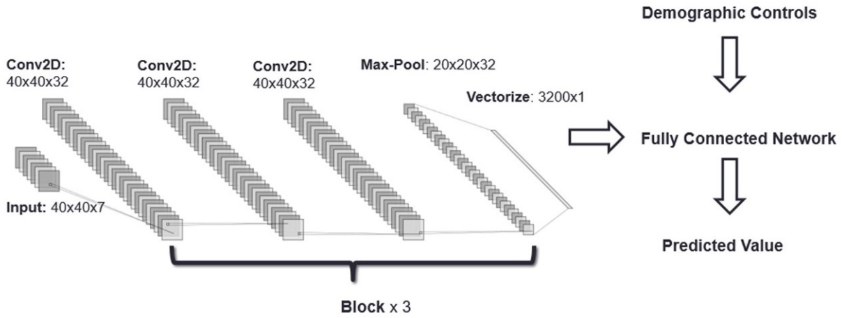
Appendix Figure 1: Convolutional Neural Network, Landsat Imagery Model Architecture
